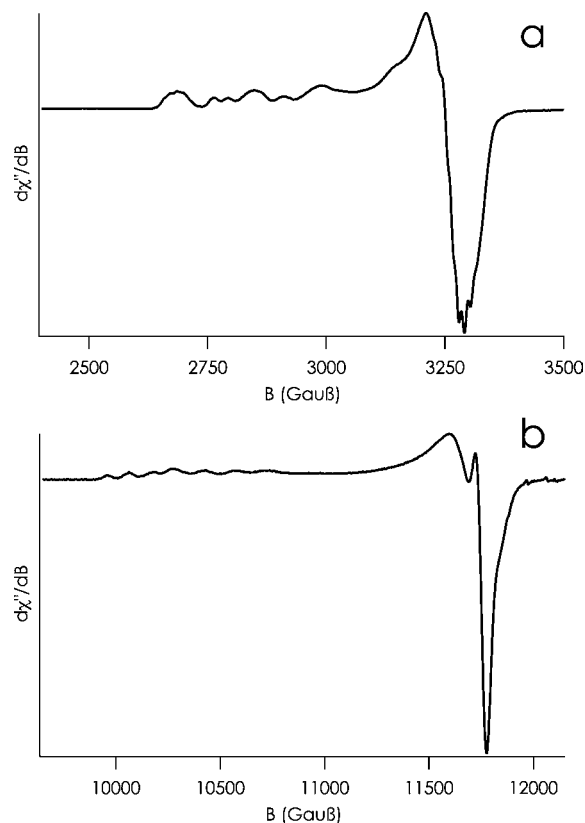
Figure 2. EPR spectra of C112D/M121E azurin recorded in aqueous 77 K glass at pH 7.0 (50 mM HEPES) at (a) X-band (conditions: frequency 9.43992 GHz; power 2 mW; modulation 6 G) and (b) Q-band (conditions: frequency 33.9476 GHz; power 3.03 mW; modulation 6 G).
