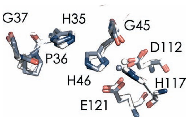
Figure 8. C_\alpha structural alignment of C112D/M121E azurin at pH 7.0 (2.1 Å, a, PDB ID: 3NP3, white) with the structure solved at pH 9.0 (2.25 Å, b, PDB ID: 3NP4, slate).
