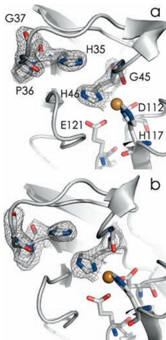
Figure 7. Active-site region showing the H35–P36 interaction in C112D/M121E azurin at pH 7.0 (2.1 Å, a, PDB ID: 3NP3) and pH 9.0 (2.25 Å, b, PDB ID: 3NP4). 2F_o - F_c maps are displayed at the 1\sigma level. Nitrogen atoms are blue; oxygen atoms are red.
