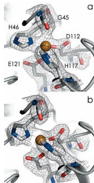
Figure 6. \text{Cu}^{\text{II}} active-site region C112D/M121E azurin at pH 7.0 (2.1 Å, a, PDB ID: 3NP3) and pH 9.0 (2.25 Å, b, PDB ID: 3NP4). 2F_o - F_c maps are displayed at the 1\sigma level. Nitrogen atoms are blue; oxygen atoms are red.
