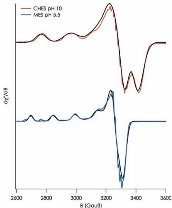
Figure 3. X-band EPR spectra of C112D/M121E azurin in pH 5.5 (blue, conditions: MES buffer; frequency 9.43997 GHz; power 2 mW; modulation 6 G) and pH 10.0 (red conditions: CHES buffer; frequency 9.43955 GHz; power 2 mW; modulation 6 G) aqueous 77 K glass. SPINCOUNT25 simulations of each spectrum are overlaid in gray.
